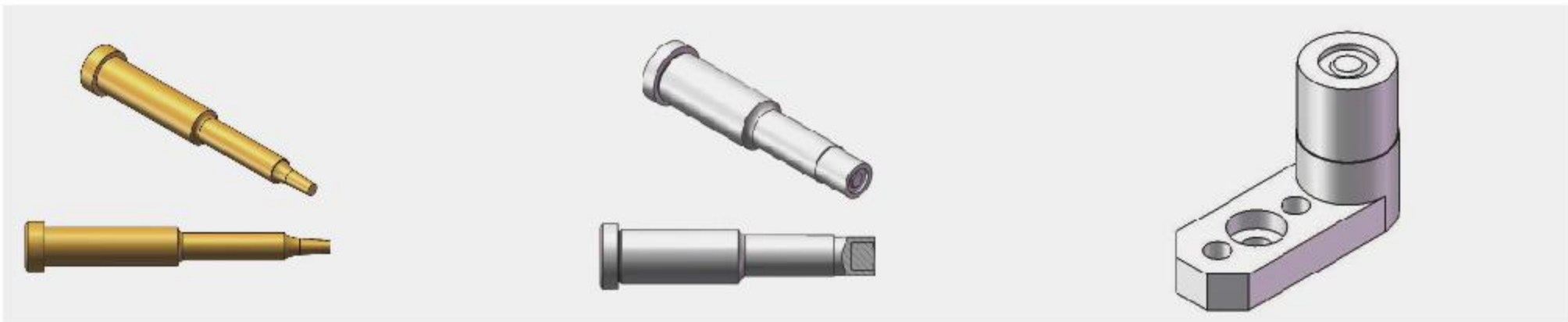
凸模 (Flanged Punch) 凹模 (Round Joint flanged die) 直角凹模 (Round Joint Die, offset)
